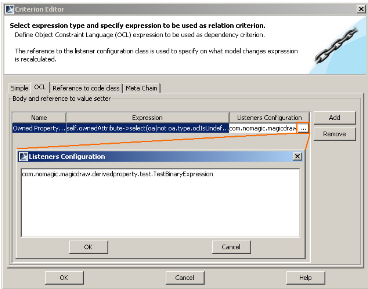
Figure 27 -- A reference to the event listener in the OCL expression
