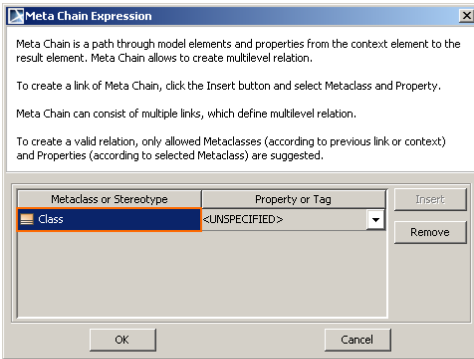
Figure 34 -- Meta Chain Expression dialog for defining links of a meta chain expression
