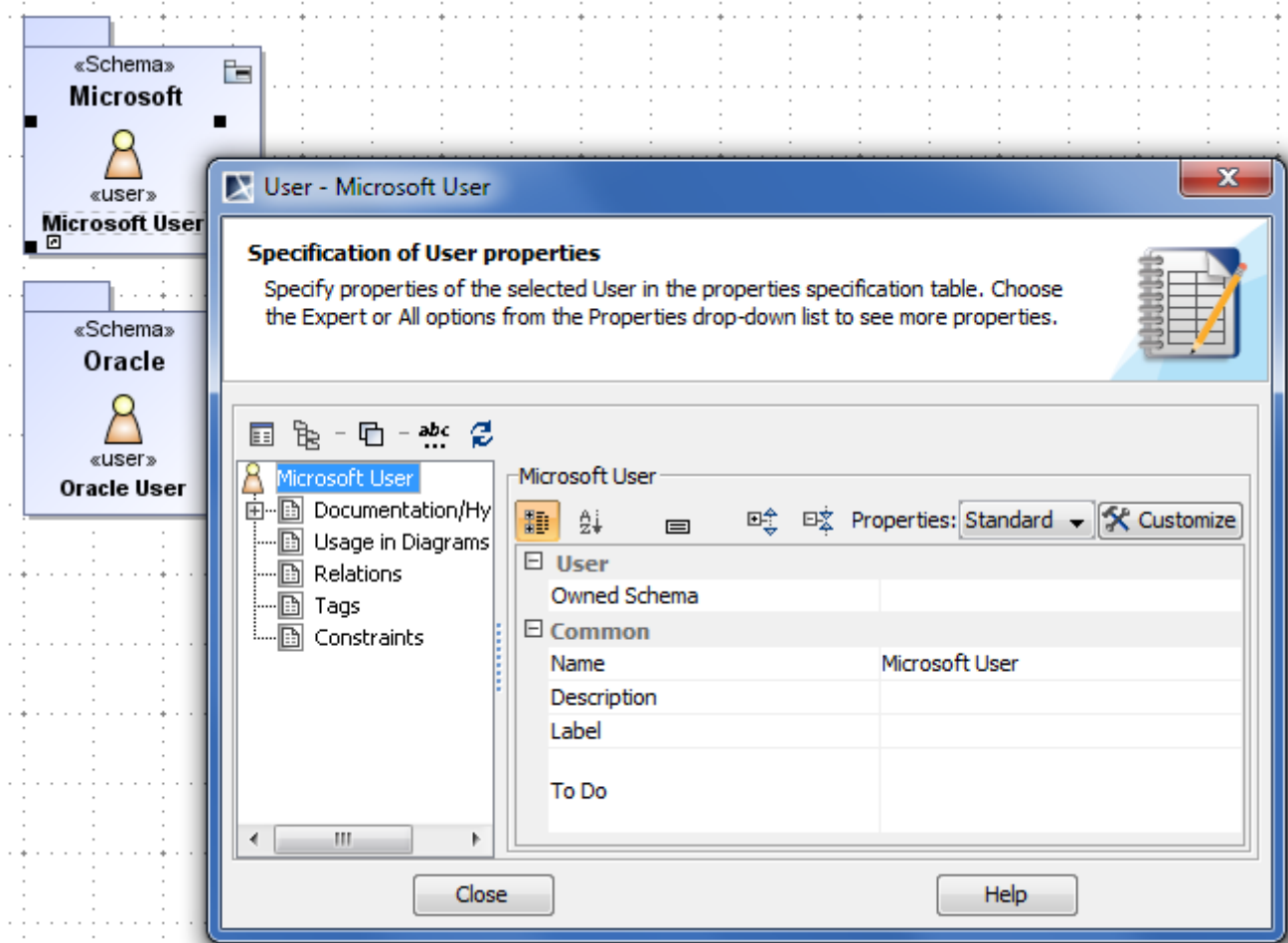
Figure 13 -- Specification window of user that is NOT INSIDE Oracle schema
