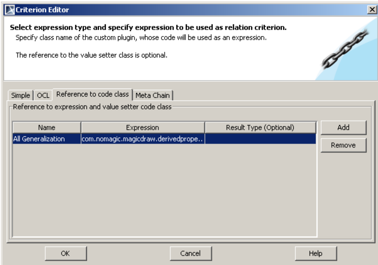
Figure 30 -- Criterion Editor dialog for defining binary expressions
