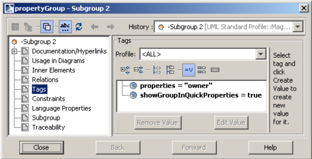
Figure 8 -- The Tags tabs of the properties "Subgroup 2"
