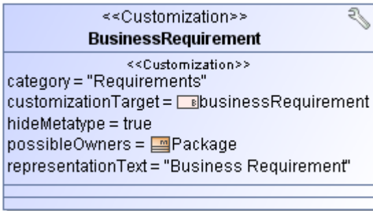
Figure 15 -- The BusinessRequirement class
