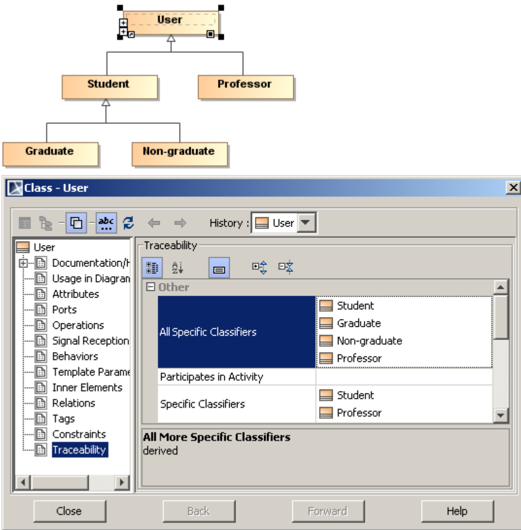
Figure 32 -- Values of the All Specific Classifiers property
