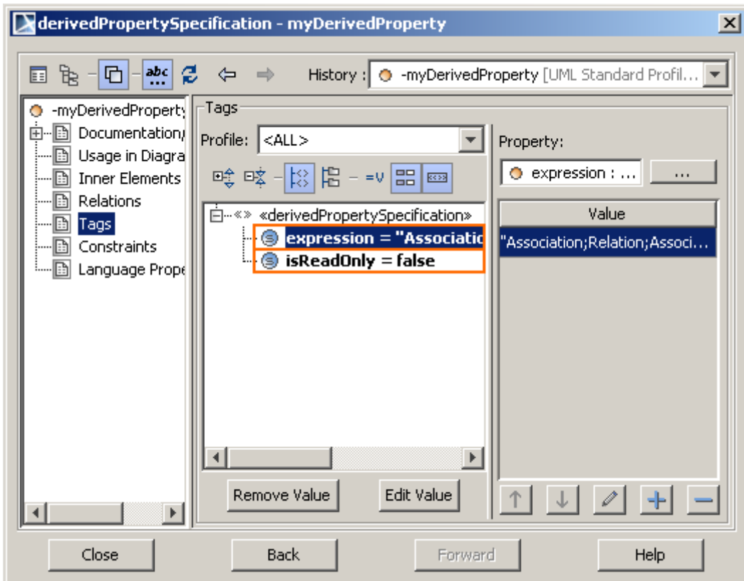
Figure 21 -- Derived property specification. Tags specification pane
