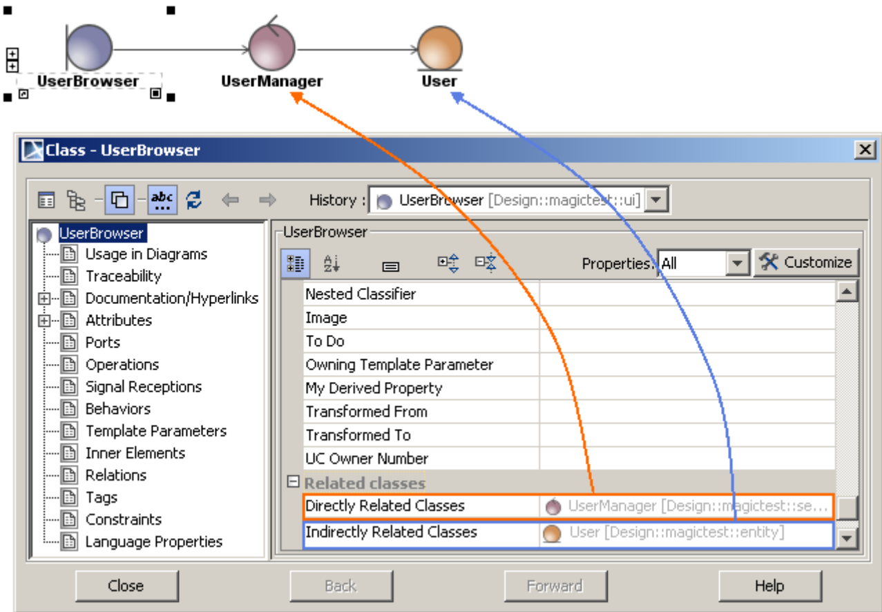
Figure 37 -- A Directly Related Classes and Indirectly Related Classes derived property values in the extended element's Specification window
