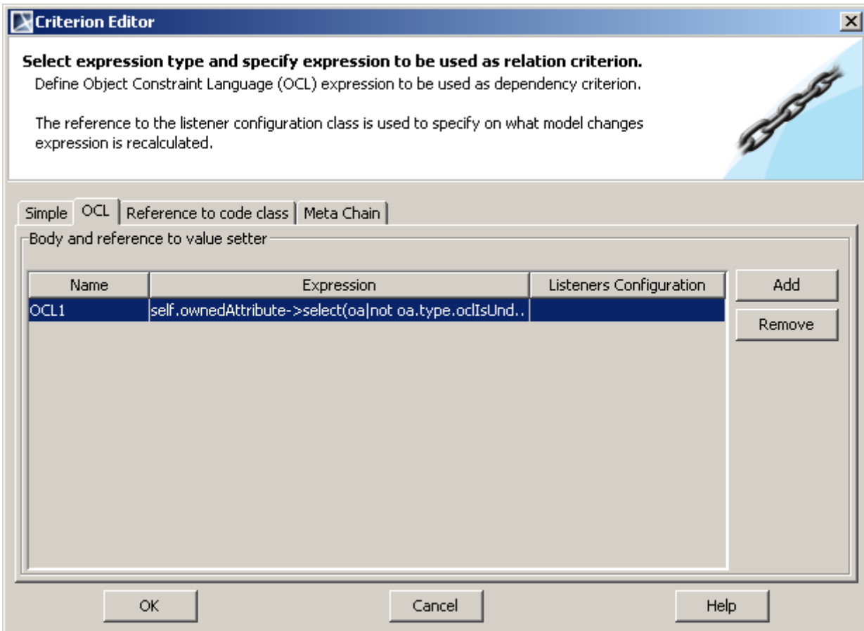
Figure 25 -- Criterion Editor dialog for defining OCL expressions
