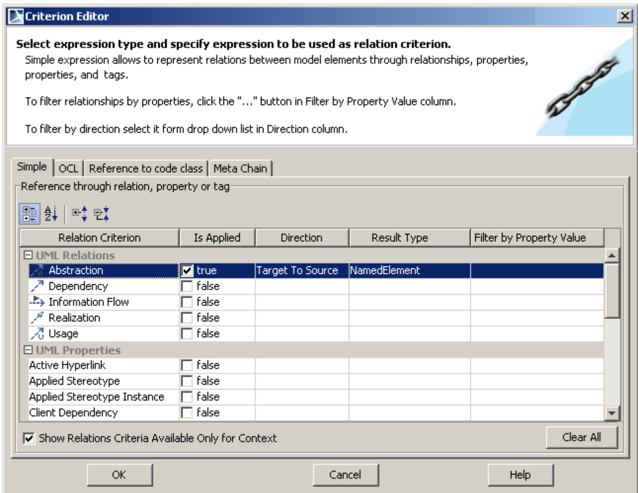
Figure 22 -- Criterion Editor dialog for defining simple expressions
