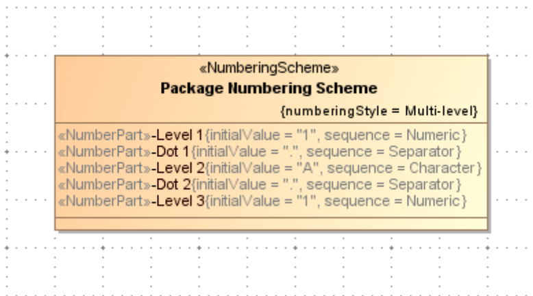
Figure 49 -- Numbering scheme with all number parts defined
