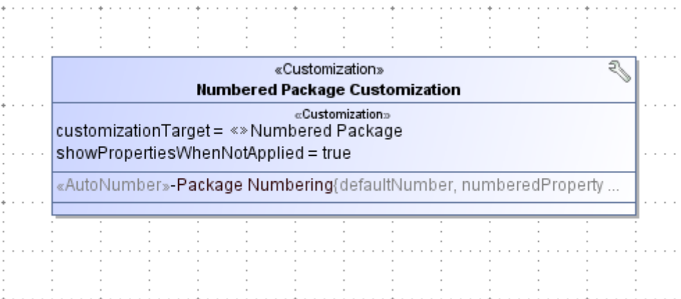
Figure 51 -- Numbering property in customization class of the “Numbered Package” stereotype
