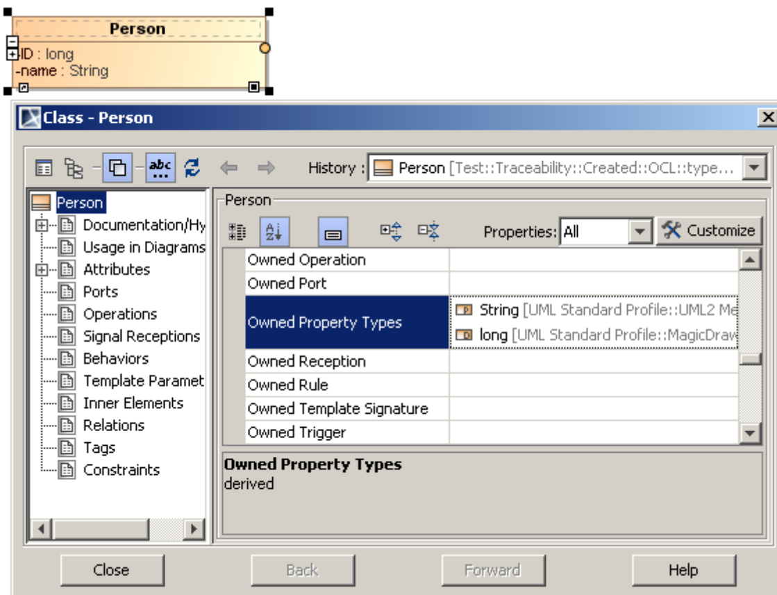
Figure 28 -- Values of the Owned Property Types property before the update of the "Person" class
