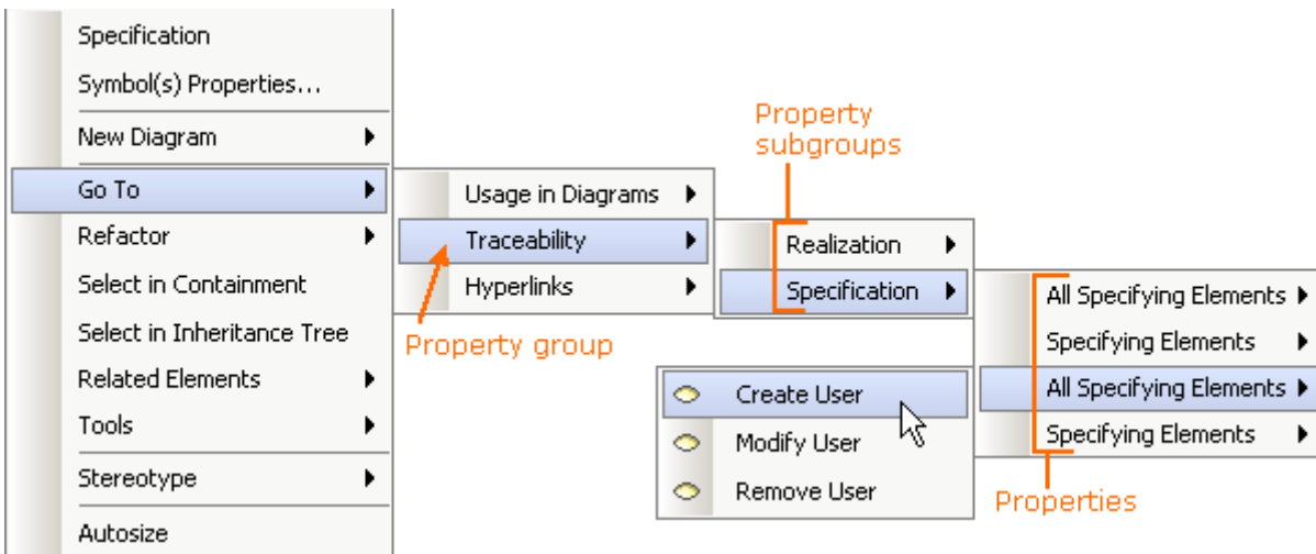
Figure 4 -- Property groups and subgroups in the element's shortcut menu
