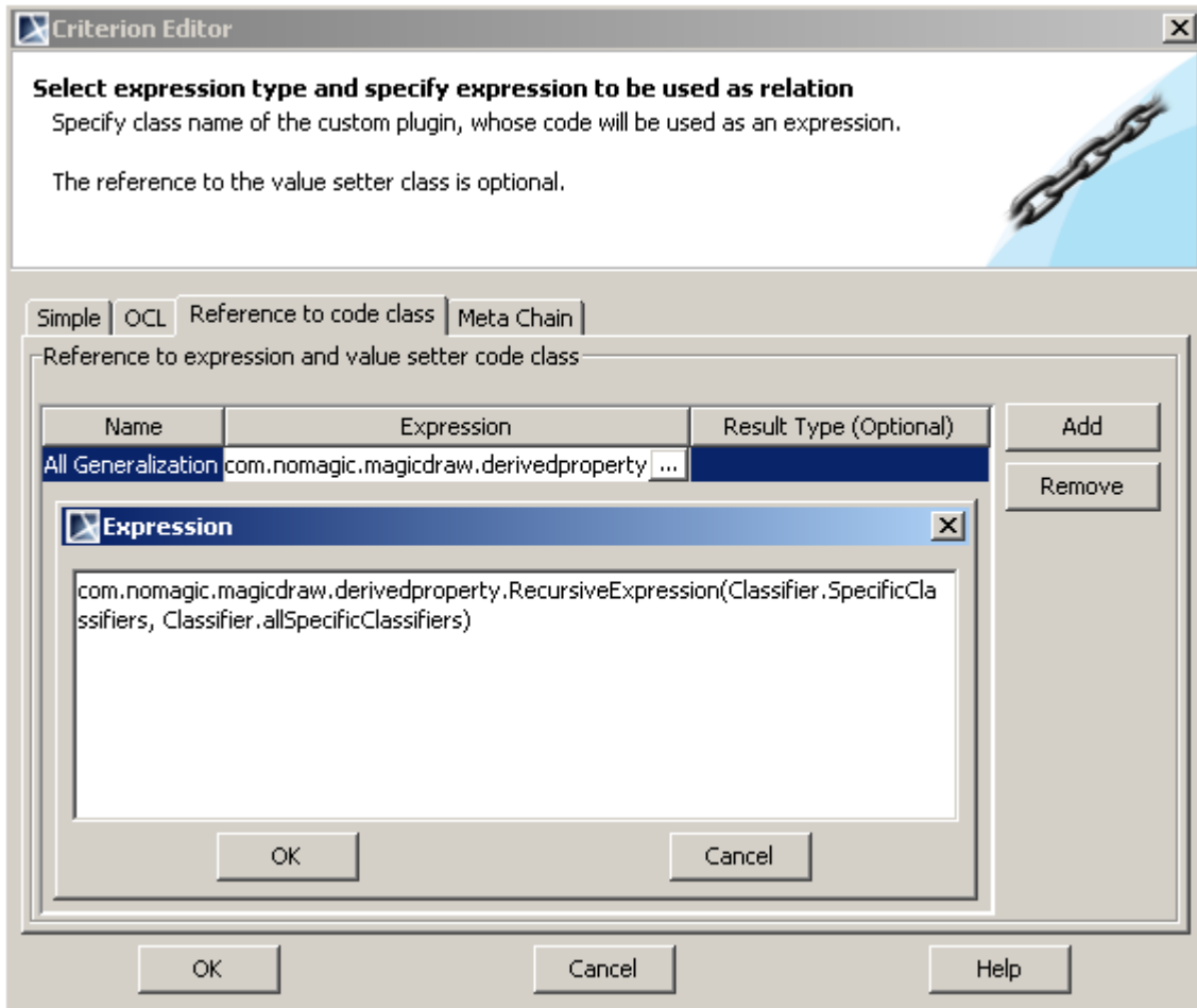
Figure 31 -- An binary expression for the All Specific Classifiers derived property
