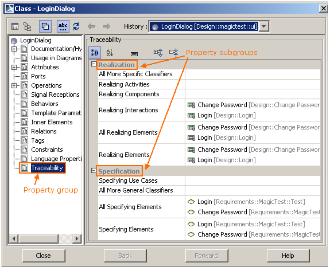
Figure 3 -- Property groups and subgroups in the element's Specification window
