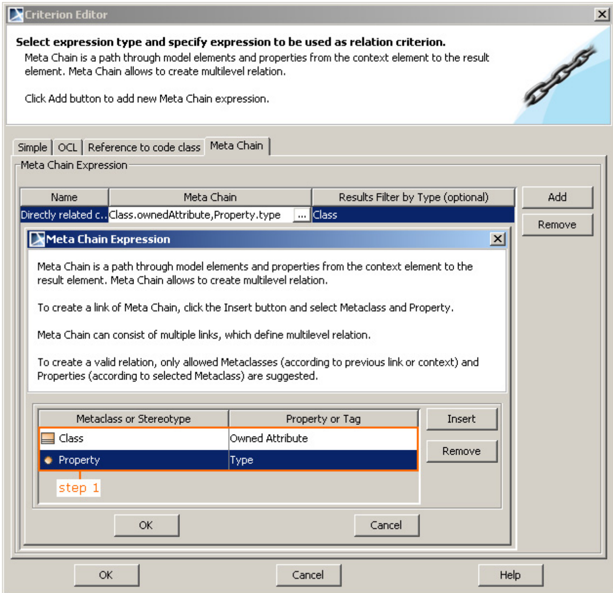
Figure 35 -- A meta chain expression for the Directly Related Classes derived property (one step)
