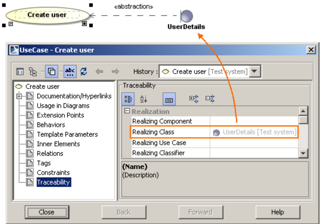
Figure 24 -- A Realizing Class derived property value in the extended element's Specification window
