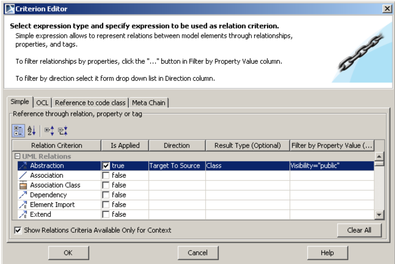
Figure 23 -- A simple expression for the Realizing Class derived property
