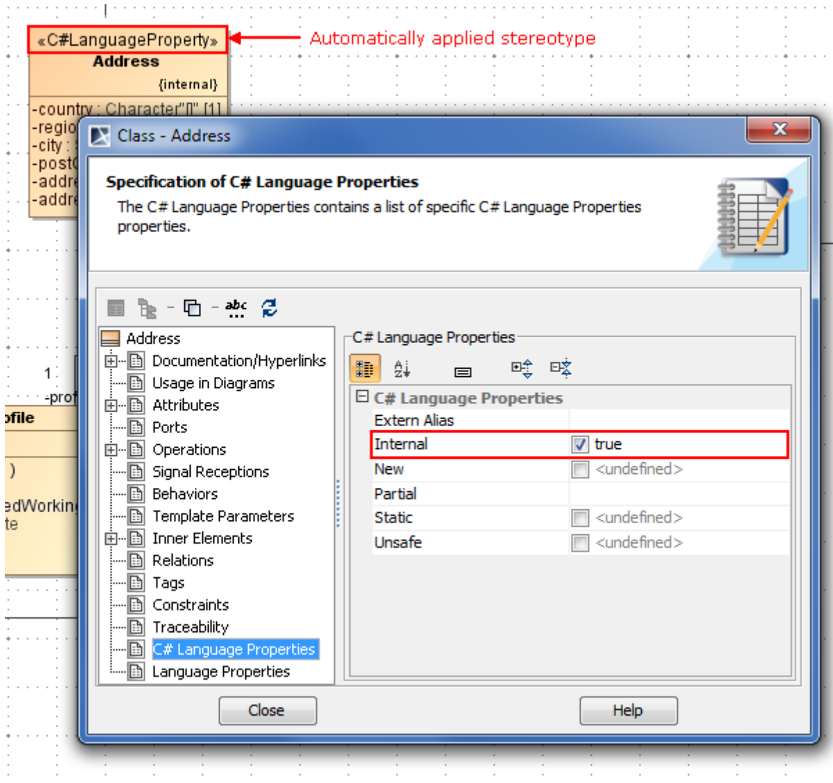
Figure 11 -- Class with automatically applied «C#LanguageProperty» stereotype
