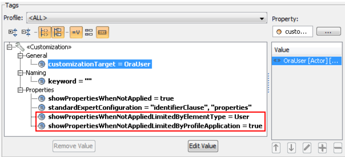
Figure 12 -- Tags for specifying advanced cases of properties visibility in «OraUser» stereotype customization class
