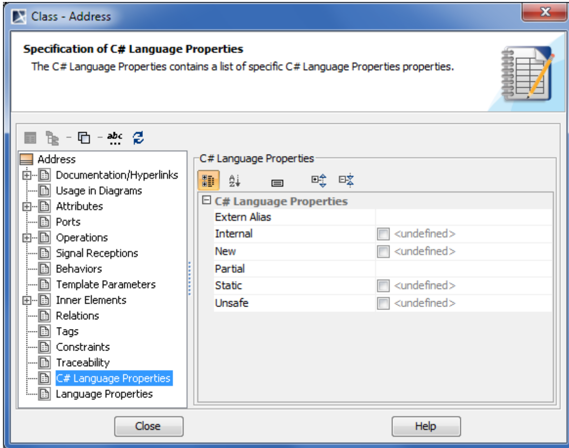
Figure 10 -- C# properties in class Specification window
