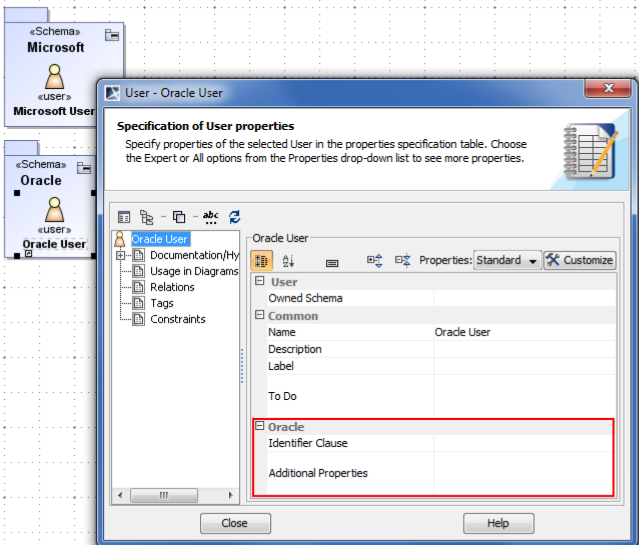
Figure 14 -- Specification window of user that is INSIDE Oracle schema
