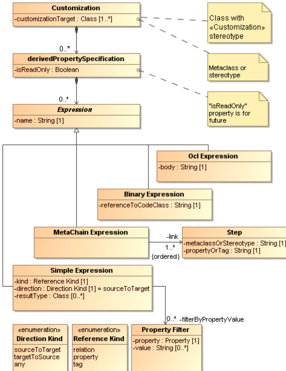
Figure 18 -- Derived properties specification metamodel
