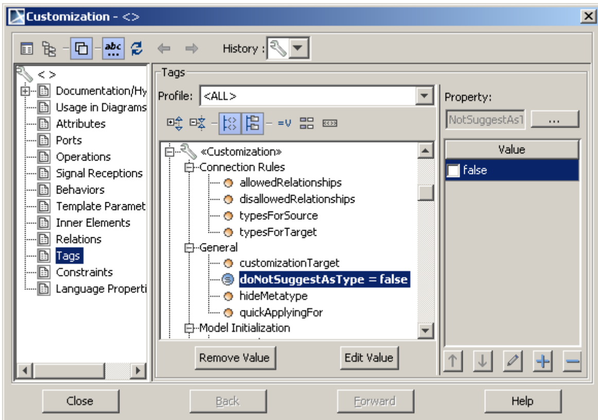
Figure 17 -- The Customization Specification Dialog, Tags branch
