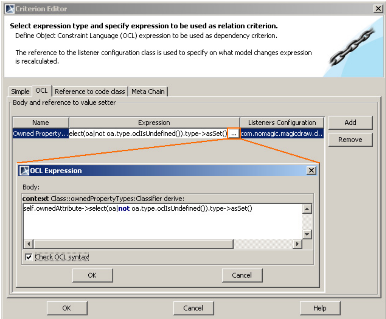
Figure 26 -- An OCL expression for the Owned Property Types derived property
