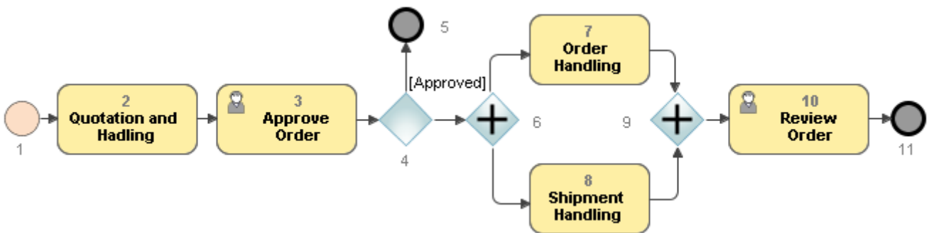
Figure 41 -- Numbering instances of different BPMN elements in sequence
