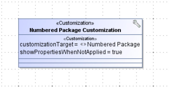
Figure 50 -- Customization class for “Numbered Package” stereotype
