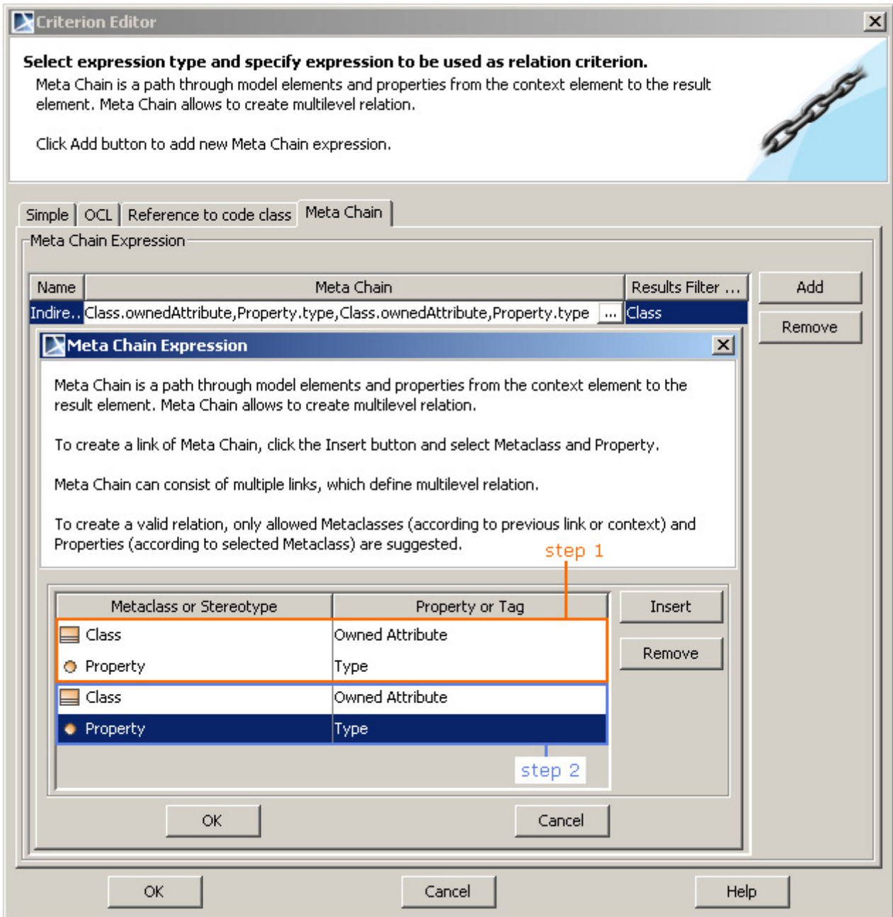
Figure 36 -- A meta chain expression for the Indirectly Related Classes derived property (two steps)
