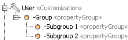
Figure 5 -- An example of customization class with the attributes for property grouping and subgrouping
