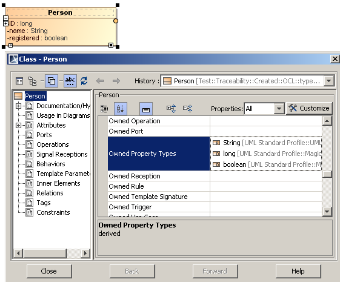
Figure 29 -- Values of the Owned Property Types property after the update of the "Person" class
