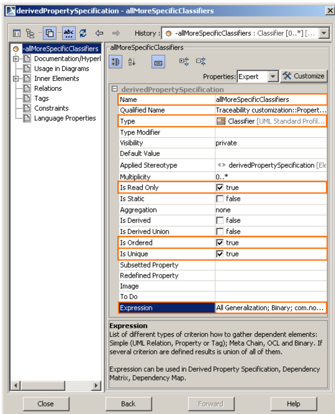
Figure 20 -- Derived property specification. General specification pane
