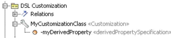
Figure 19 -- An example of the customization class with the attribute for the derived property specification
